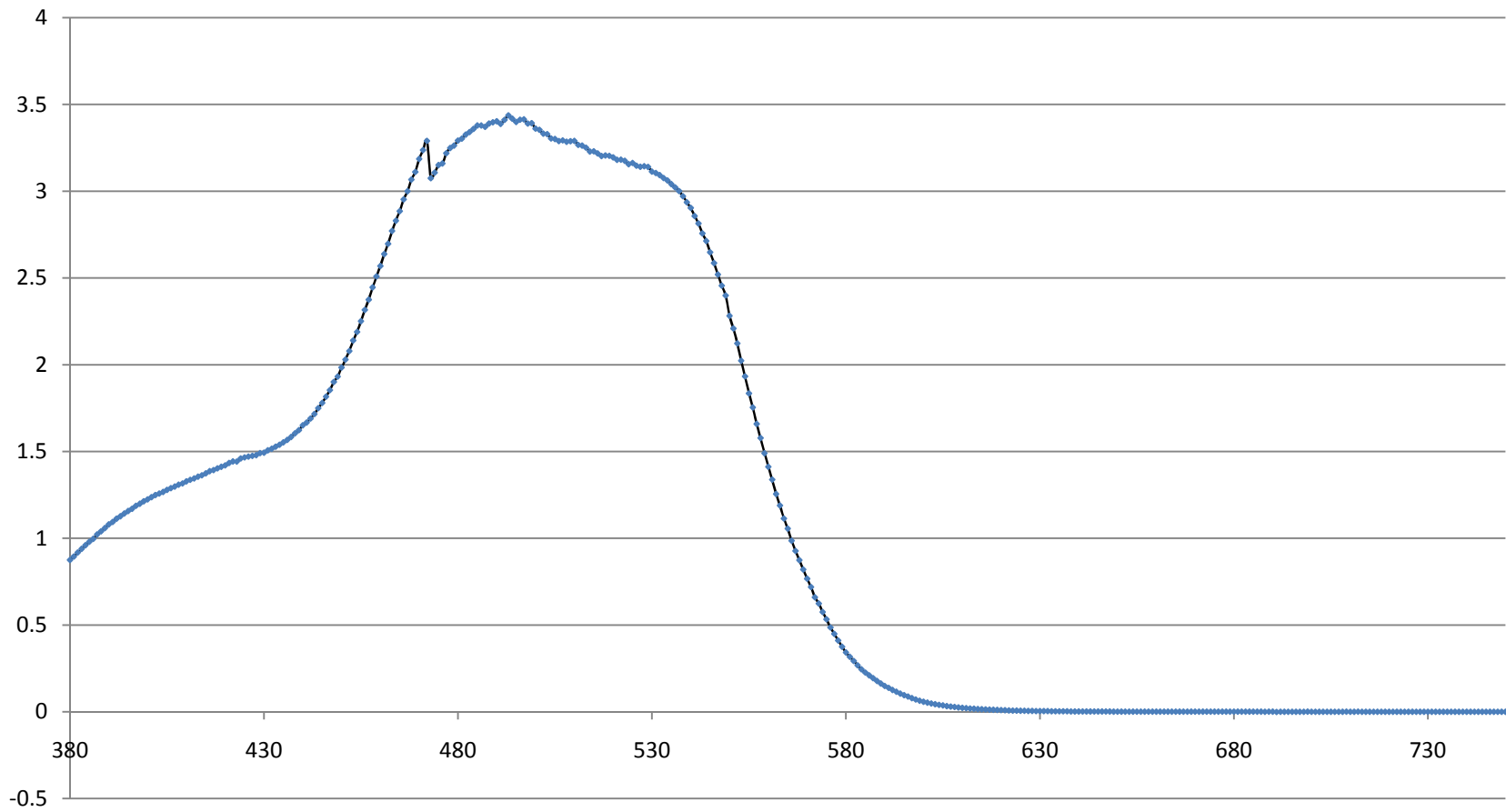
Figure 1. Absorbance spectrum for red food dye used in photosynthesis experiment.
