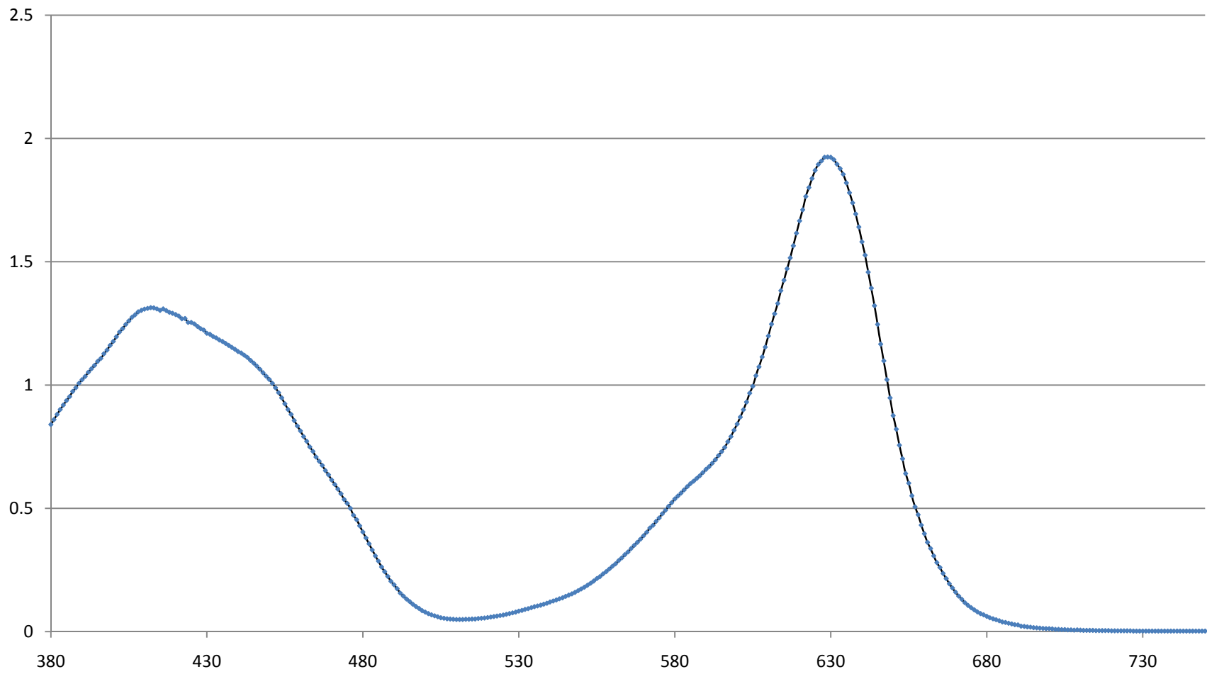
Figure 2. Absorbance spectrum for green food dye used in photosynthesis experiment.
