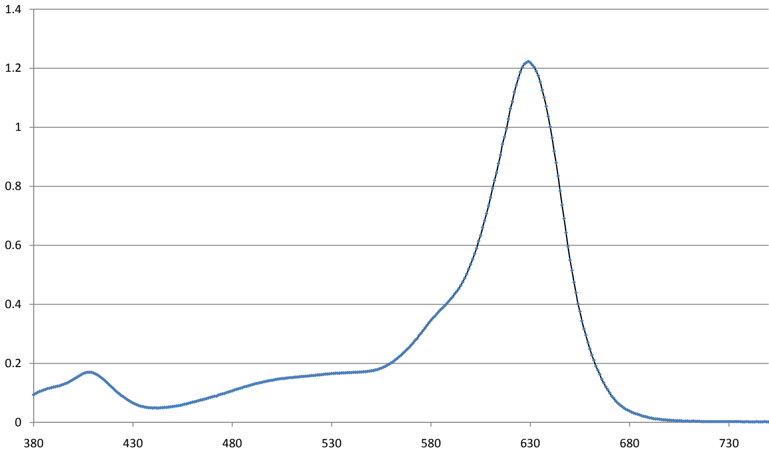
Figure 3. Absorbance spectrum for blue food dye used in photosynthesis experiment.
